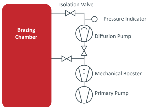
Typical layout for vacuum brazing
